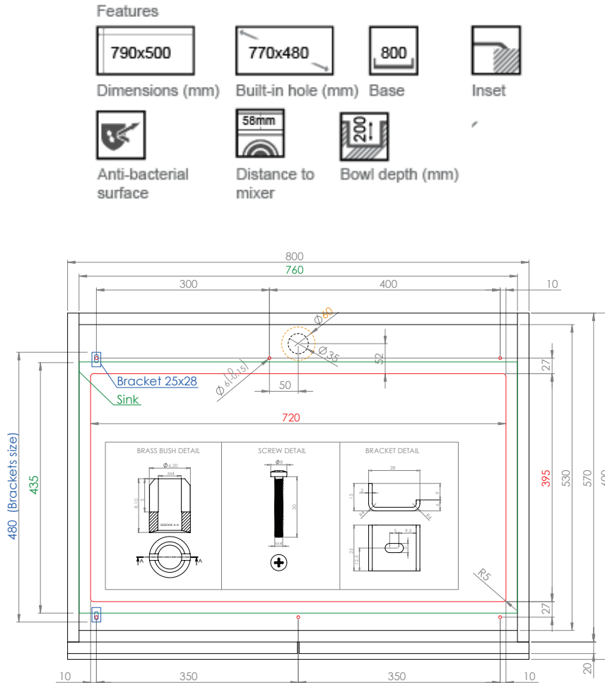
Technical data sheet Quadra 350 Under Mount
