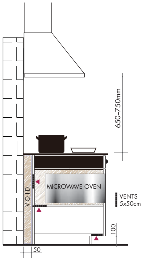
VENTILATION REQUIREMENTS FOR UNDERBENCH INSTALLATION
